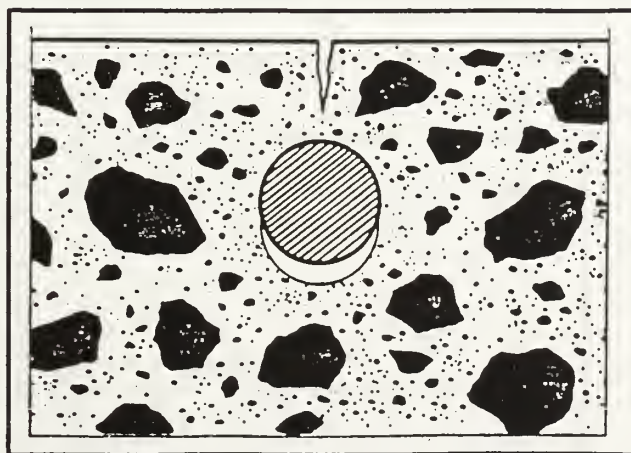
Figure 2.6 Obstructed settlement crack. (Reference 4)
